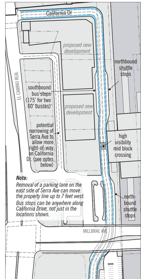
FIGURE 7-6. California Drive Extension Plan View
