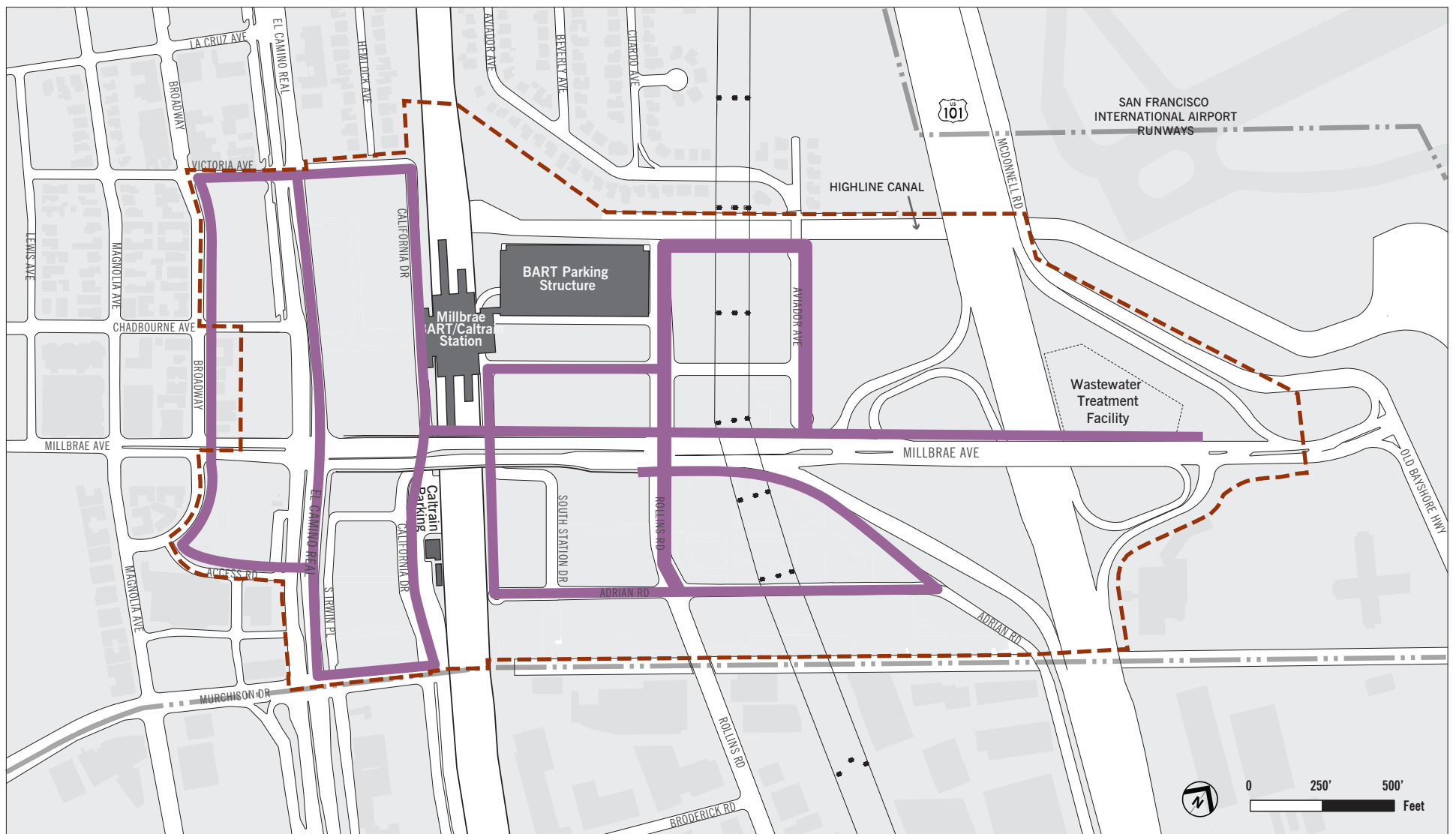
FIGURE 8-2. Proposed Recycled Water System
