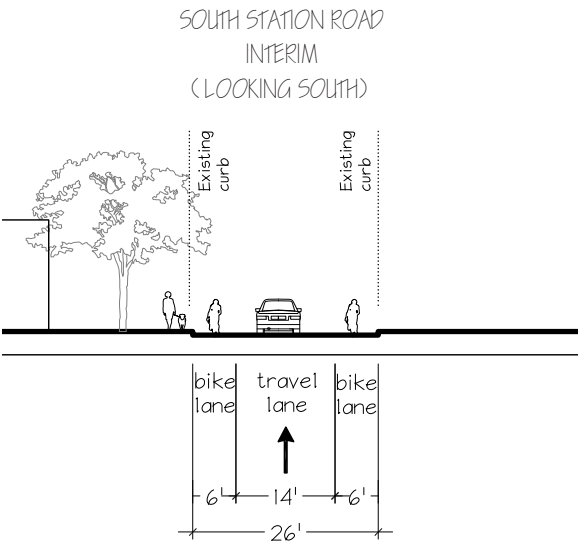
FIGURE 7-9. South Station Road (Interim) Typical Section
