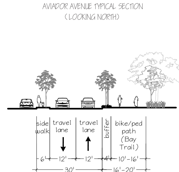
FIGURE 7-12. Aviador Avenue Typical Section
