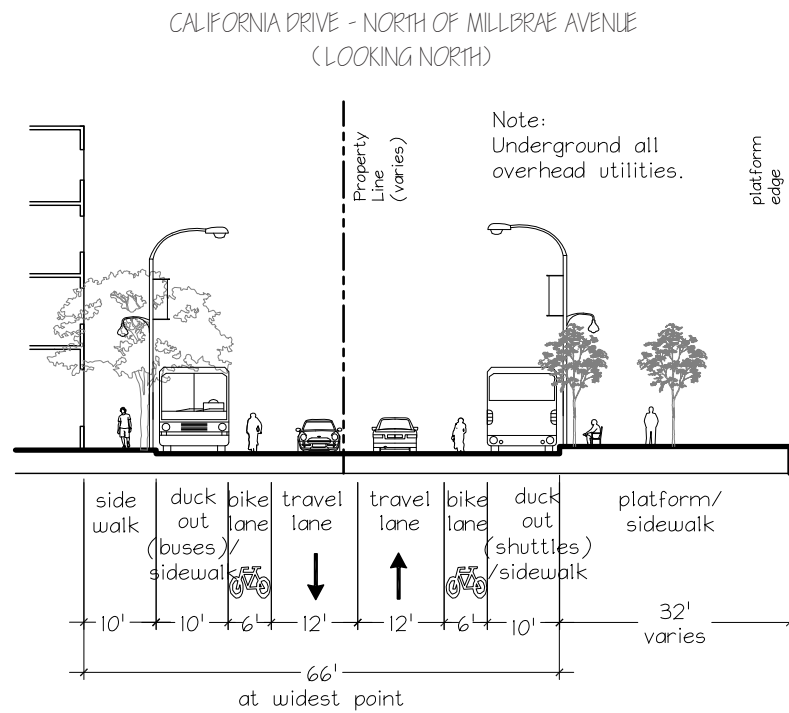
FIGURE 7-7. California Drive Typical Section
