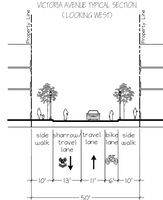
FIGURE 7-11. Victoria Avenue Typical Section
