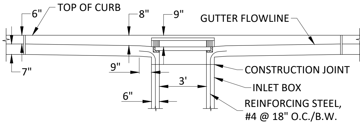
SECTION A-A INLET AT NORMAL CURB
